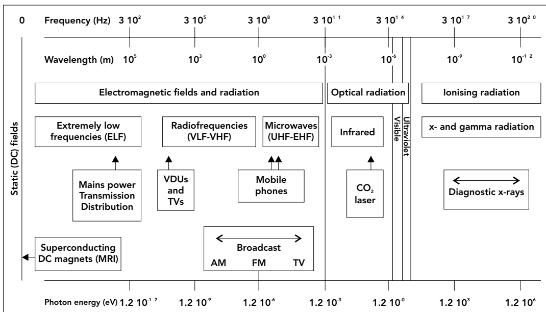
Electromagnetic spectrum
